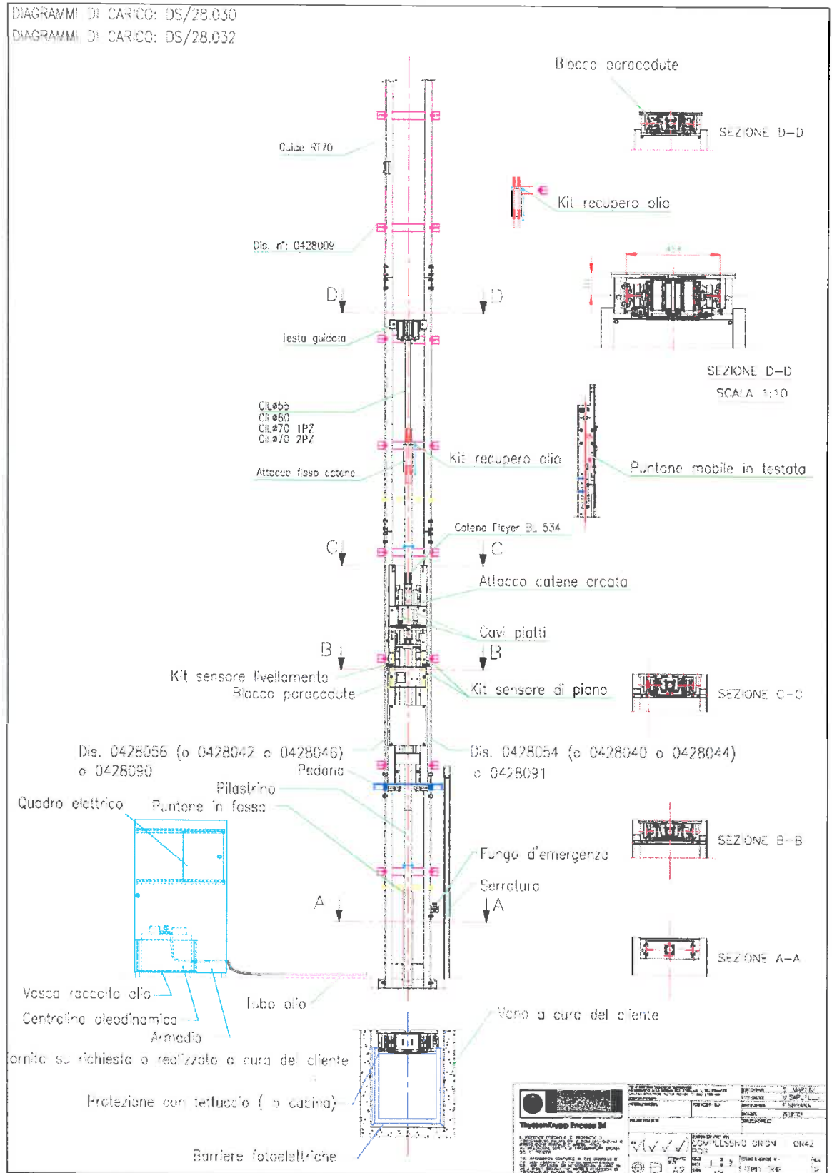
Figure 3 – General drawing ORION 42 – Close guide
